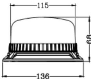
FLAT BASE
